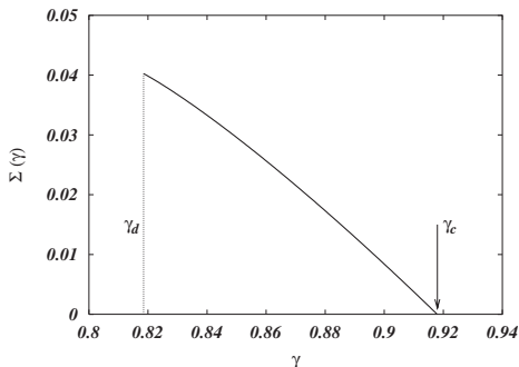
Fig. 2. The complexity as a function of \gamma .
